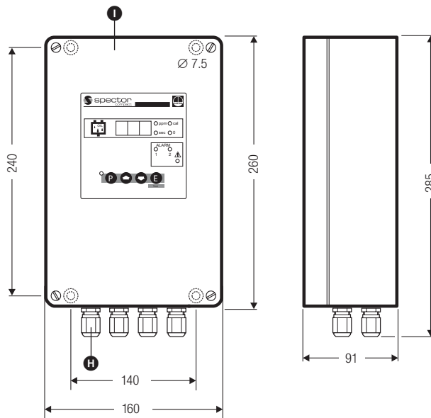
Measuring transducer ORT 6 (field case for wall mounting)
